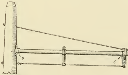
Fig. 195. One Type of Bracket for Trolley Line
